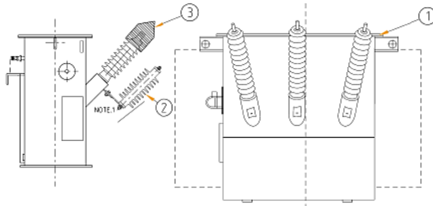
THREE PHASE - THREE BUSHING
