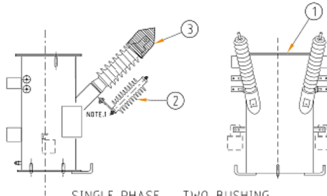
SINGLE PHASE - TWO BUSHING
