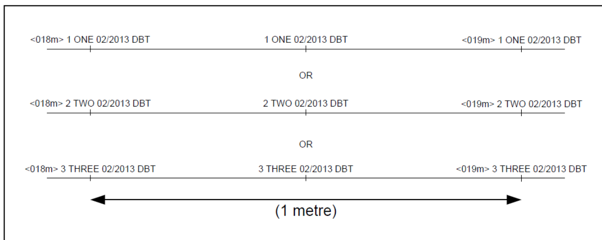
Figure 1: Cable Marking
